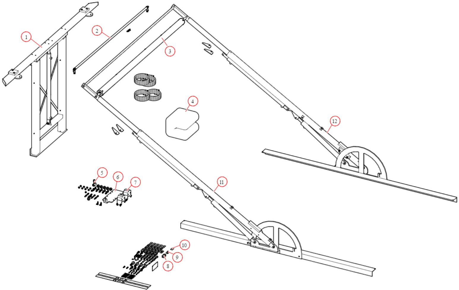
79300 (ROHGHS).Roll-Off Hydraulic Gantry / Hydraulic Slide Arms
