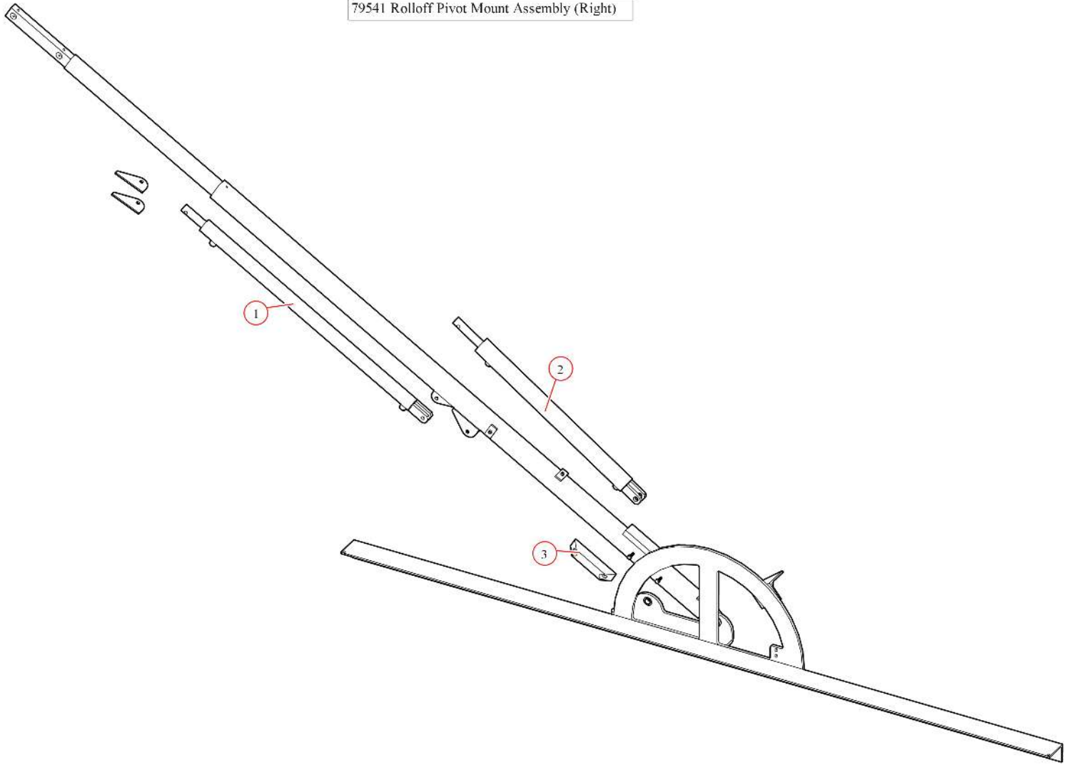
79541 Rolloff Pivot Mount Assembly (Right)
